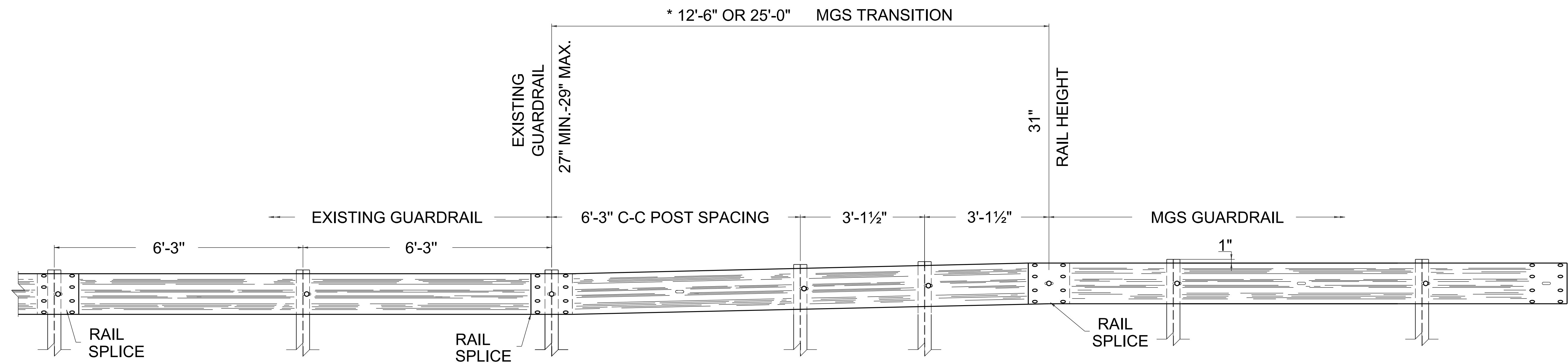
ELEVATION VIEW
